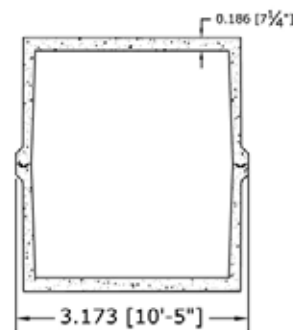
SHORT SECTION
