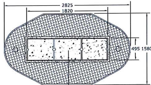
ROOF PLAN
